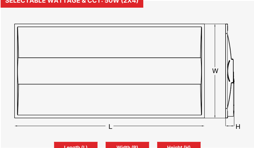
SELECTABLE WATTAGE & CCT: 50W (2X4)
